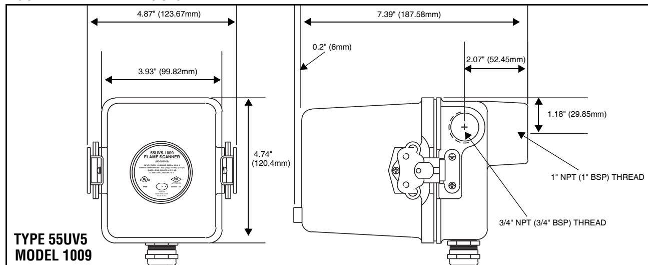
FIGURE 1. DIMENSIONS
