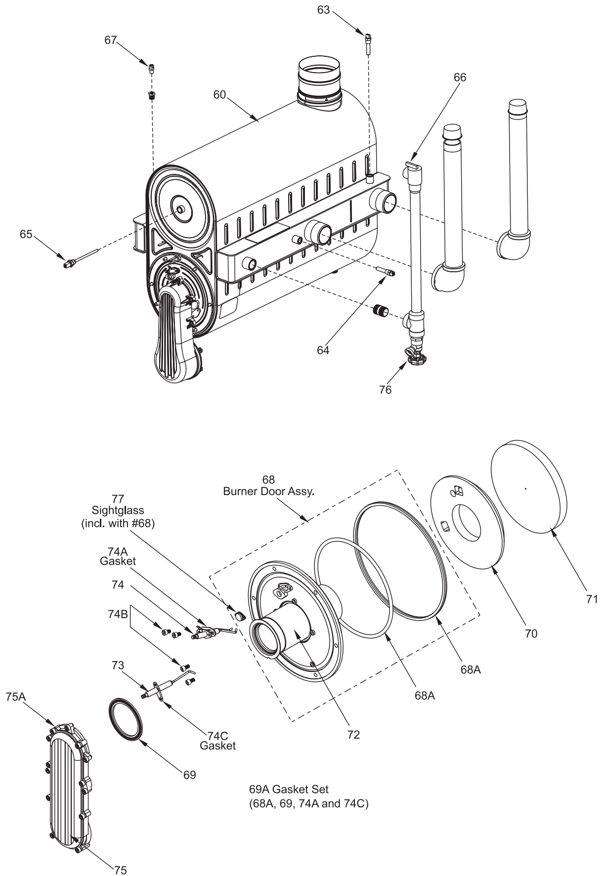
Figure 53 - Heat Exchanger Components
